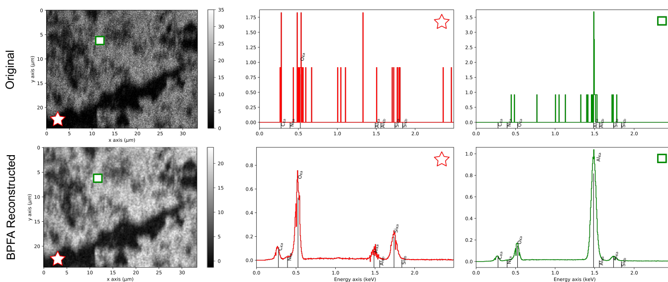
Figure 1. Results of a BPFA compressed sensing reconstruction on an SEM-EDS map of an aluminum silicate sample. The leftmost column shows the Al-K \alpha intensity map, indicating the locations of the single-pixel spectra shown in the center ( star ) and right ( square ) columns. The top row indicates the as-collected data; the bottom shows the data after BPFA reconstruction, demonstrating the substantial improvement in signal quality after reconstruction.
